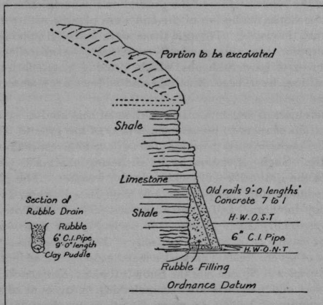
Fig 48.—Type Section of Cliff (Lyme Regis)
