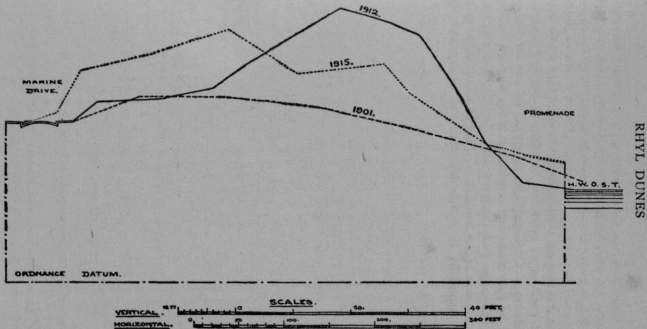
Fig. 13.—Section of Sand Dune Formation, Rhyll
